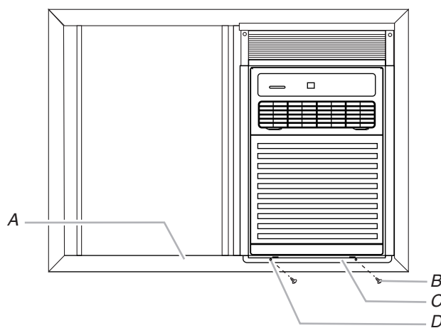
A. Window channel frame B. \frac{3}{8} " self-tapping screw C. Bottom bracket D. \frac{1}{8} " drilled hole
