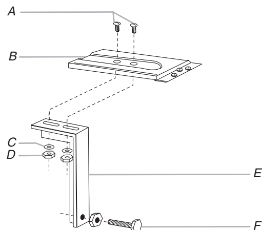
A. \frac{7}{16} " machine screws B. Support plate C. Flat washer D. Nut E. Support angle F. Leveling bolt and locknut
