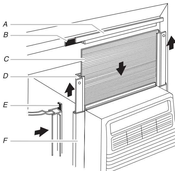
A. Top retainer B. Seal under top retainer C. Filler board
